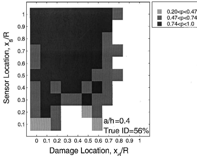
Fig. 8 Damage identification results for several damage intensities.
