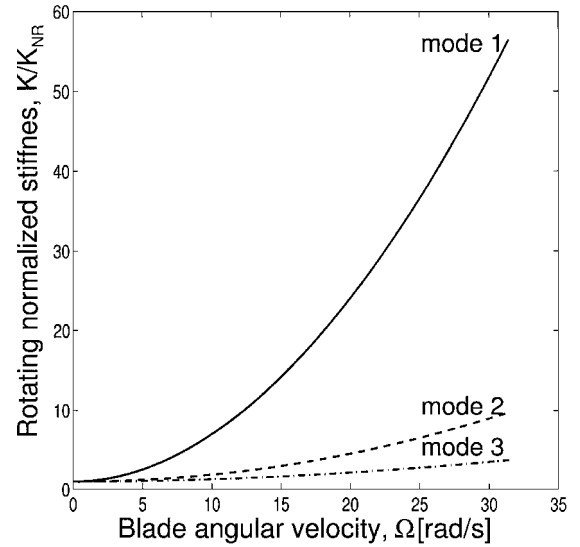
Fig. 10 Normalized modal stiffness vs blade angular velocity.
