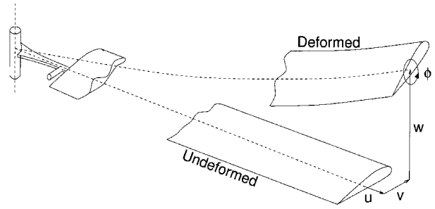
Fig. 11 Deformed elastic blade.
